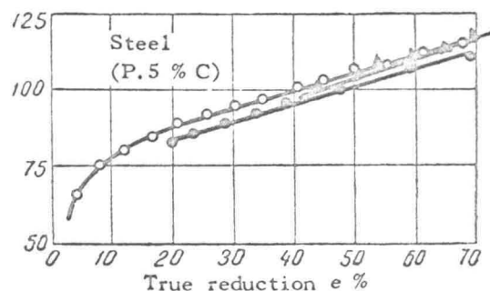
Fig. 1. Tensile test diagrams for St.50 specimens ○-○- after coldworking by elongation ( e - 15 per cent) under 3500 atm, pressure; ○-○- no coldworking; △-△- after coldworking by elongation ( e - 40 per cent) under 3500 atm, pressure.
